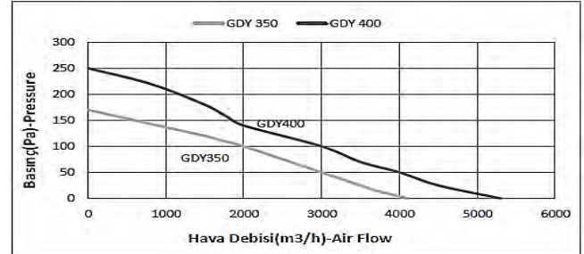
GDY350-400
