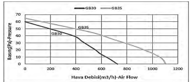
GB30-35
