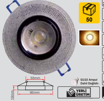
Ada Cam Spot ERK9007
