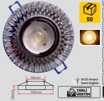
Side Cam Spot ERK9026
